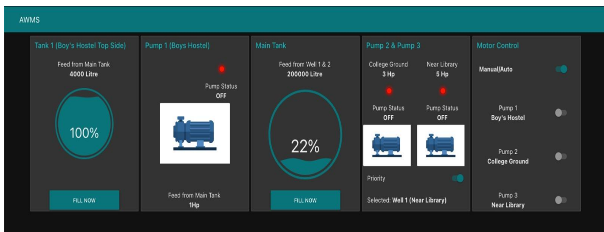
Figure 30: Water Management System Monitor
